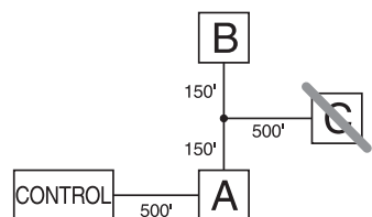
Figure 2-2 Câblage Corbus
