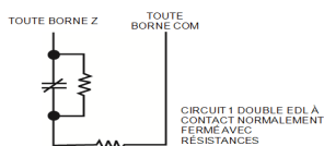
Figure 2-10 Câblage DEDL
