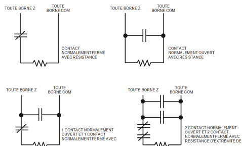
Figure 2-9 Câblage SEDL
